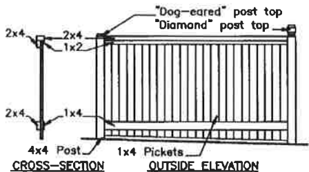
CROSS-SECTION OUTSIDE ELEVATION
