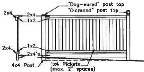
CROSS-SECTION OUTSIDE ELEVATION
